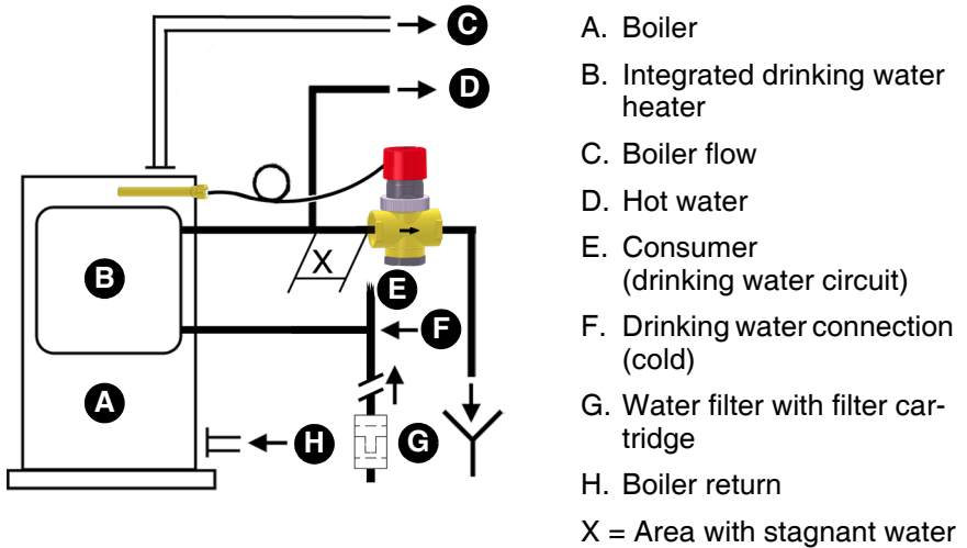
Fig. 1: Boiler with integrated drinking water heater
