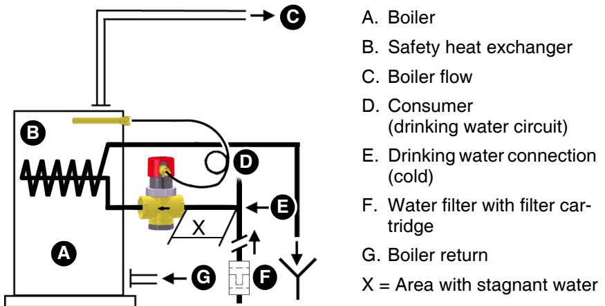
Fig. 2: Boiler with safety heat exchanger
