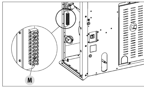
Fig. 73 - Anschlüsse
