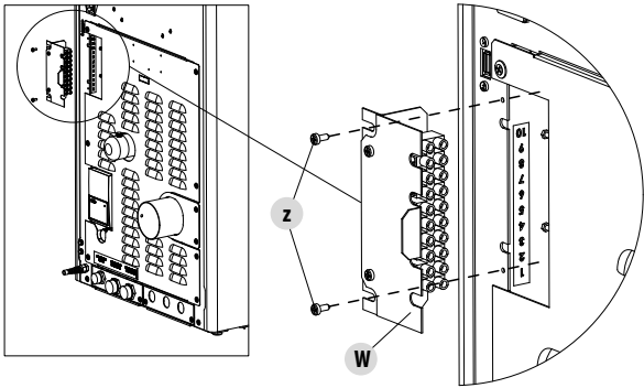
Fig. 72 - Anschlüsse
